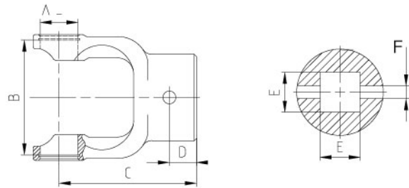
四方销孔节叉 18 Square yoke – pin hole 18
