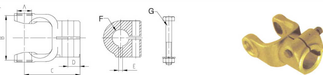
圆孔键槽夹紧螺栓叉 14 Plain bore yoke– keyway & clamp bolt 14
