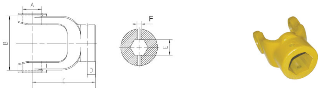
六角螺孔节叉 15 Hexagon yoke – threaded hole 15
