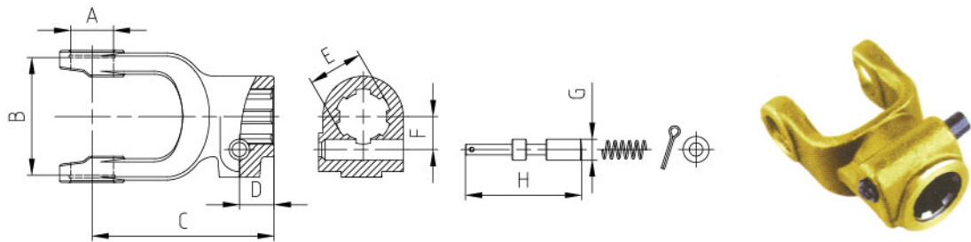
通销花键叉 07 Splined Yoke – push pin 07
